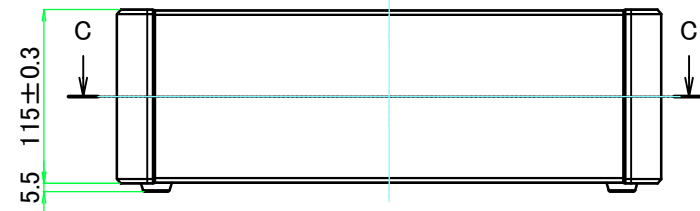
A view
