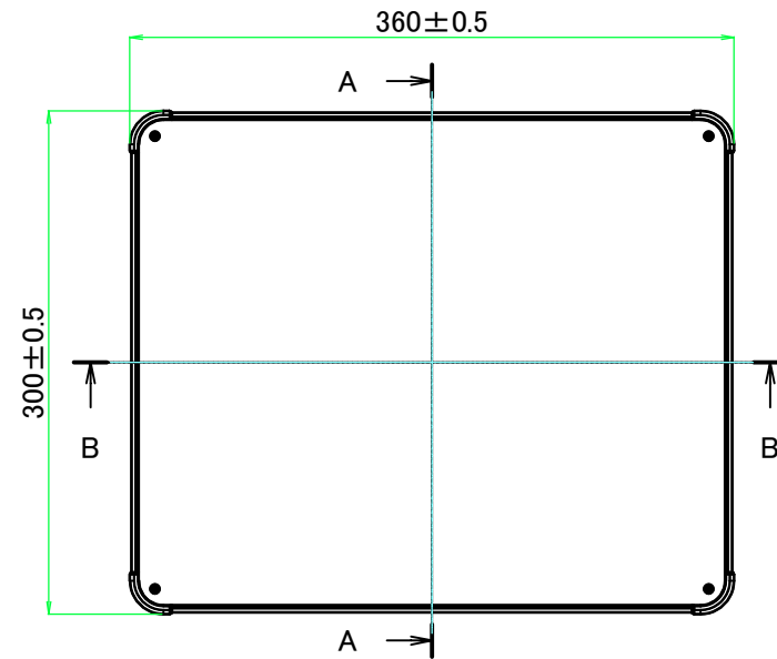
E view
